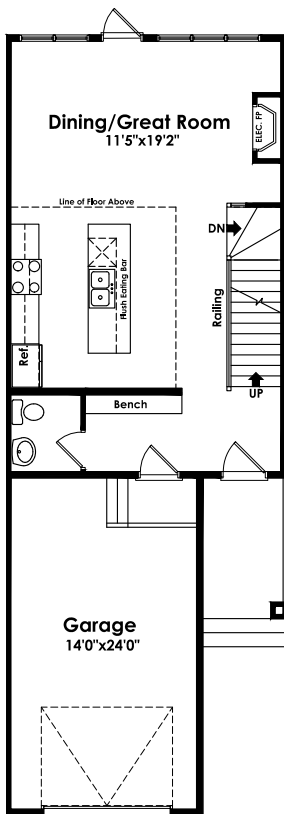
MAIN FLOOR 630 sq. ft.
