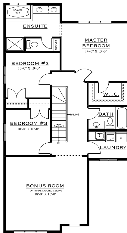
SECOND FLOOR 1,182 sq. ft.
