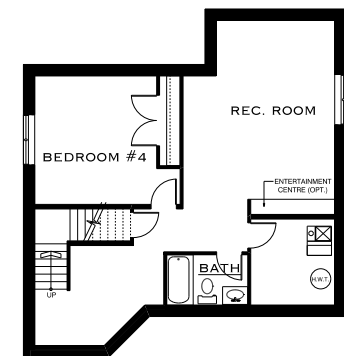
DEVELOPED BASEMENT (Option B - 705 sq. ft.)
