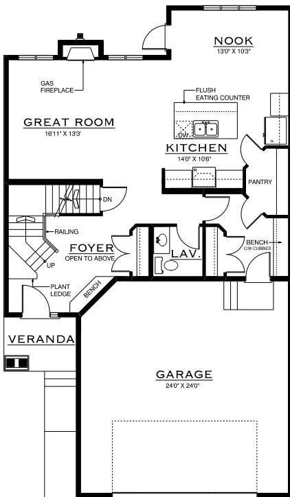
MAIN FLOOR 919 sq. ft.
